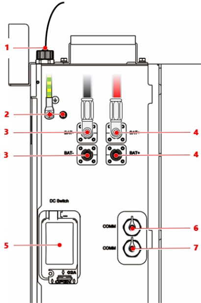
Figure 3: Battery Description
