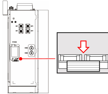
Figure 13: Turning off the circuit breaker
