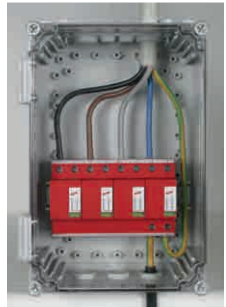
Application example: Modular DEHNventil M TNS installed in an IGA 10 V2 IP54 insulating enclosure.
