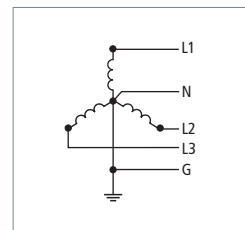
three-phase; 5 wire
