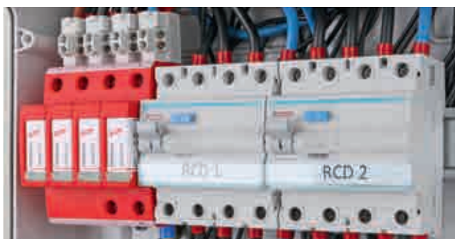
STAK 3X16 for EMC-optimized series connection of string lines in a PV generator junction box.
