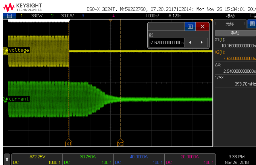
Test Category: Only the photovoltaic (PV) Reaction time: 2.54S
