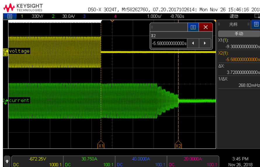
Test Category: Only the Battery Reaction time: 3.72S
