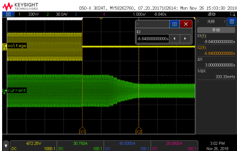
Test Category: Both batteries and photovoltaic cells Reaction time: 3S
