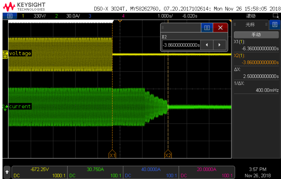
Test Category: Only the Battery Reaction time: 2.5S
