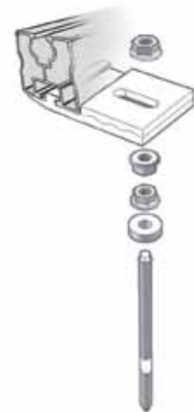
KlickTop fastening kit for corrugated roofs
