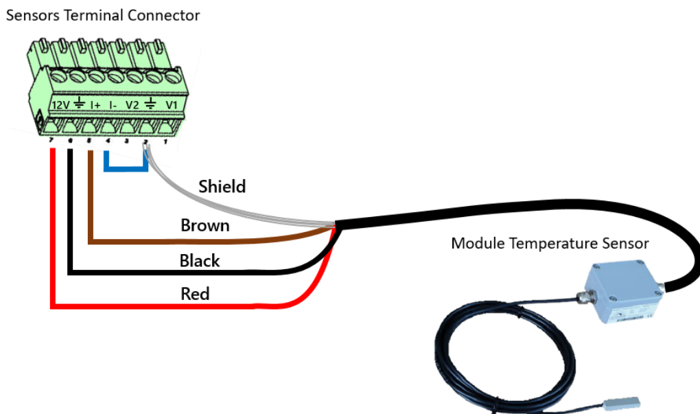
Figure 6: Connecting the Module Temperature Sensor
