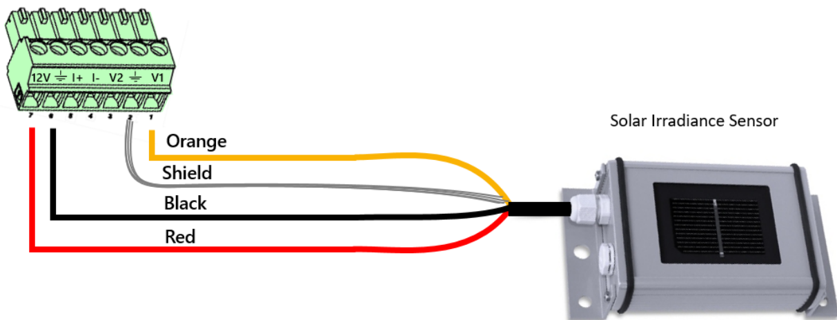
Figure 8: Connecting the Solar Irradiance Sensor
