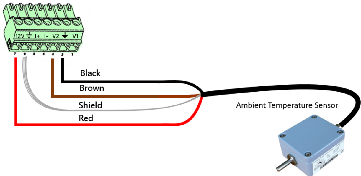
Sensors Terminal Connector
