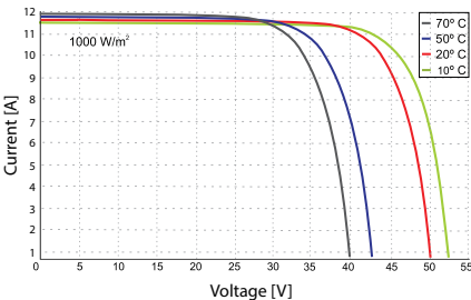
I-V Curve at Various Cell Temperatures
