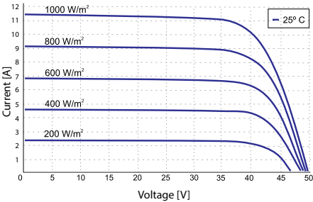
I-V Curve at Various Irradiation Levels
