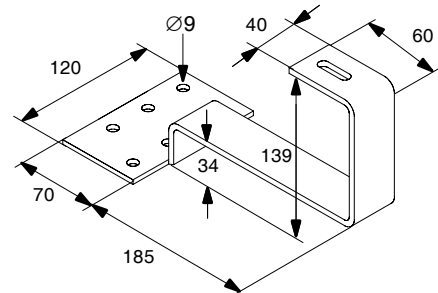
Roof anchors Pantile-6
