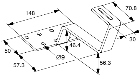
Roof anchors Pantile-5
