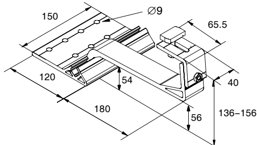
Roof anchors Pantile-4-AI
