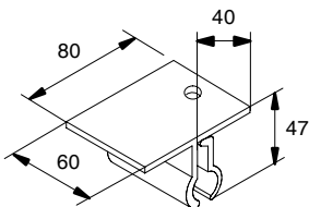
Beam clip
